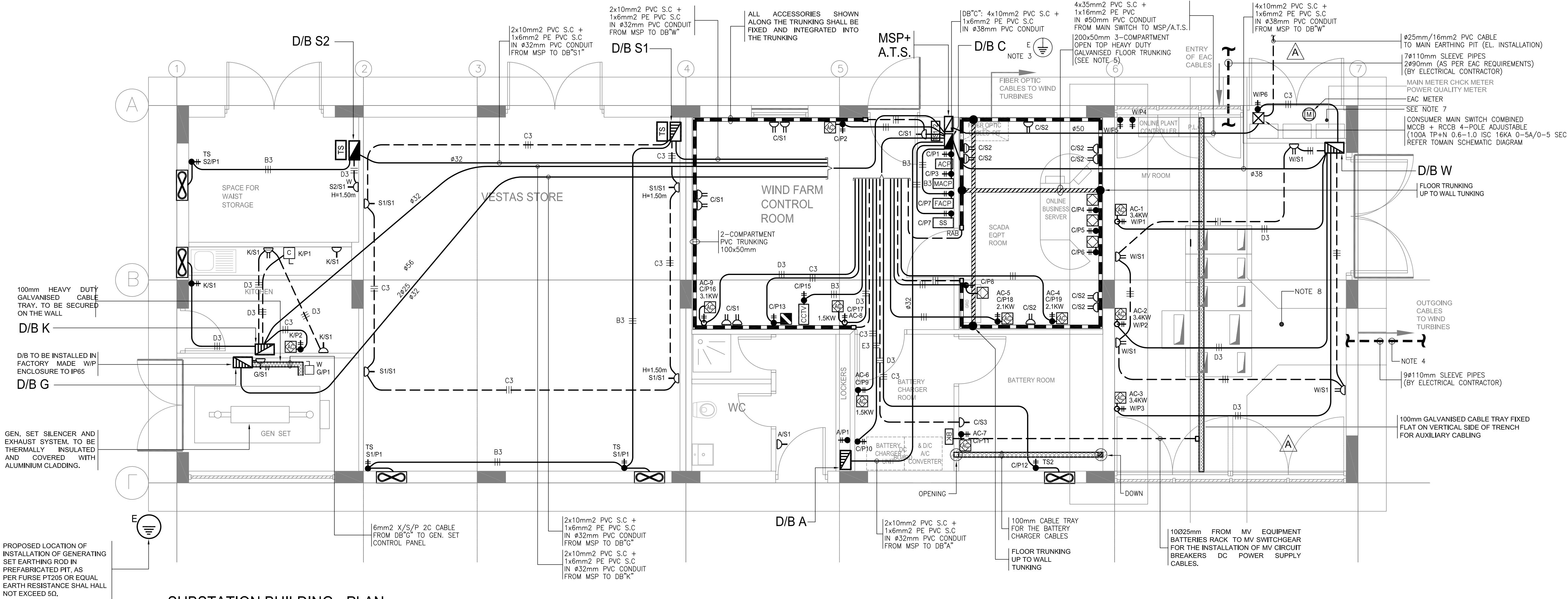
SUBSTATION BUILDING - PLAN SMALL POWER INSTALLATIONS SCALE 1:50
